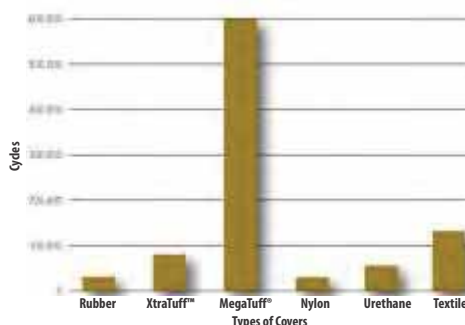
Teste de Abrasão / Prueba de Abrasión ISO6945 — Metal-to-hose rubbing cycles to lose one gram of weight
